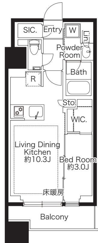
D type 1LDK 35.95㎡
