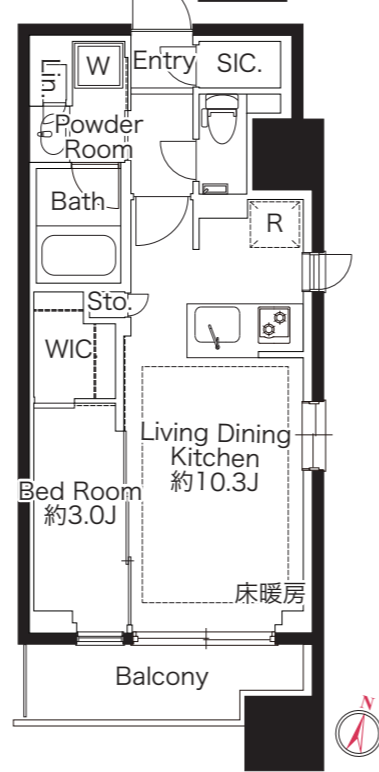
C type 1LDK 35.89㎡
